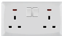
K10-W025 2* 13A switched socket with neon(DP)
